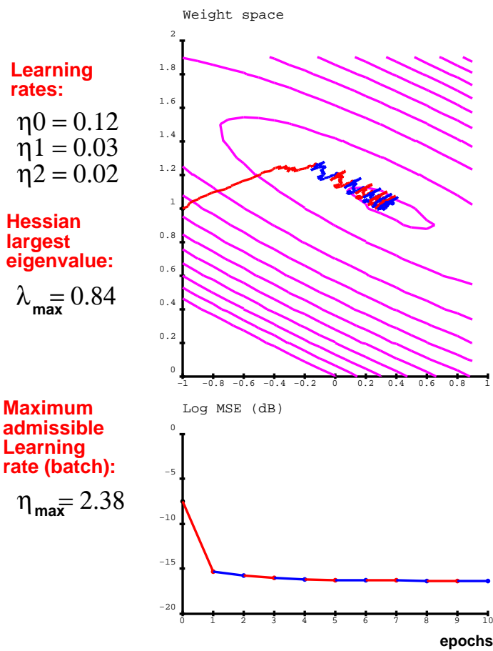
Fig. 22. Stochastic diagonal Levenberg-Marquardt algorithm. Data set from 2 Gaussians with 100 examples. The network has one linear unit, 2 inputs and 1 output, i.e. three parameters (2 weights, 1 bias).
