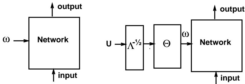
Fig. 15. Sketch of the whitening properties of the Newton algorithm.
