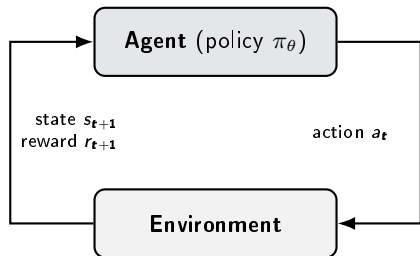
The agent–environment loop (Sutton & Barto).
