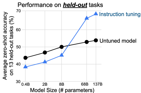
Zero-shot accuracy on held-out task types vs. model size (FLAN, Wei et al., 2022).
